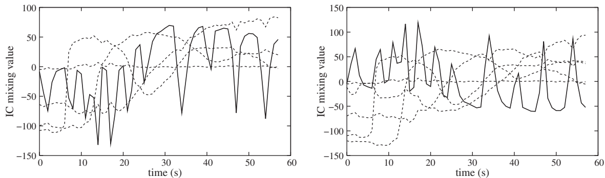
Fig. 6. Left: Mixing matrix obtained using a five component ICA. Note, that the shape of the quasi-periodic movement component indicates that it is not completely separated from the perfusion component. With a six component ICA this effect is reduced significantly (right).
