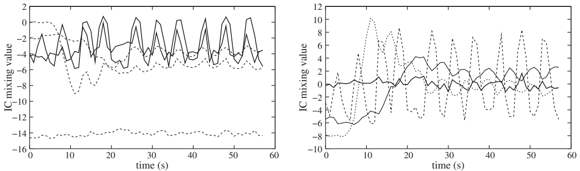
Fig. 5. Left: Mixing matrix obtained using a five component ICA. Note, that the quasiperiodic movement component is actually split into two components. Using a four component ICA results in better separation (right).
