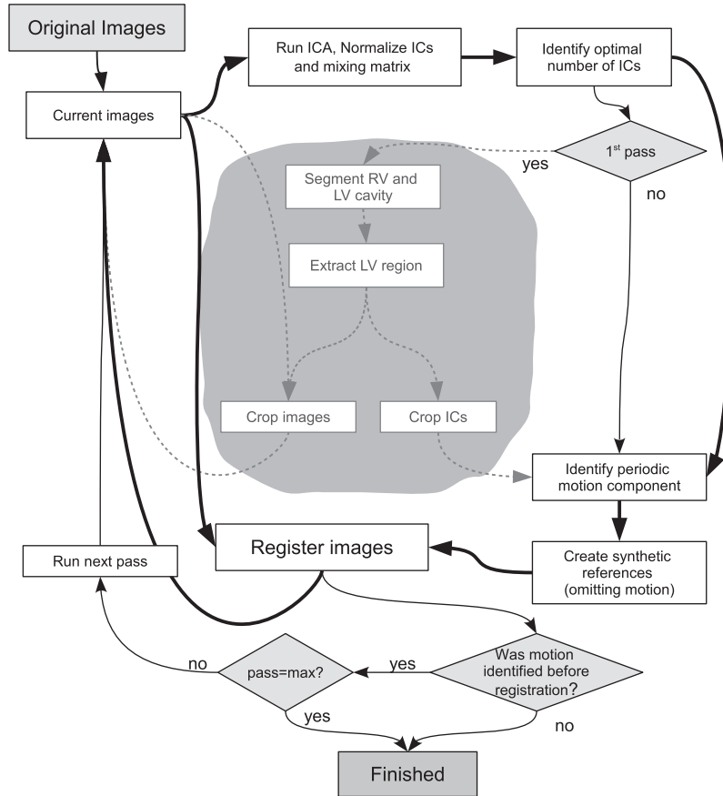
Fig. 4. Scheme of the registration algorithm. The bold lines indicate the data flow and the thin lines represent the logical flow. The grayed texts in the gray area and dashed lines represent the additional steps for bounding box creation that are not a requirement for a non-linear motion compensation scheme. These steps may be executed to accelerate the registration and are required if linear registration is to be run.
