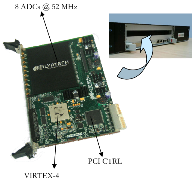
Fig. 2: Photo of the actual acquisition board and chassis, with the SBC in place.
