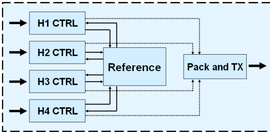
Fig. 2: Diagram of the coincidence unit architecture
