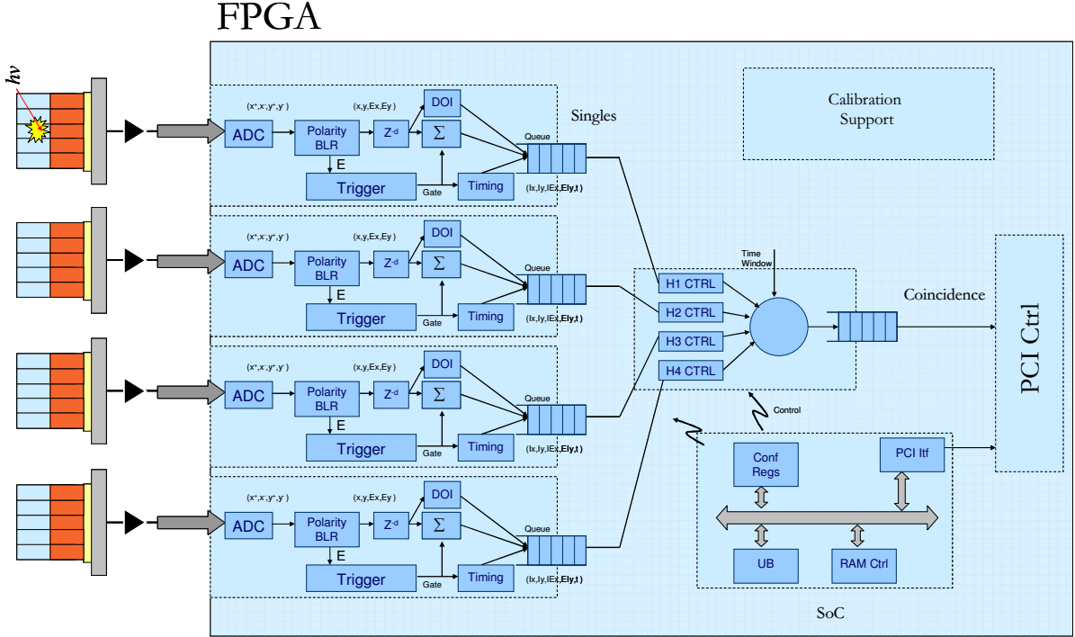
Fig. 1: Diagram of the on-chip architecture, including four single processors, one coincidence sorter and on-chip block (SoC) for slow control
