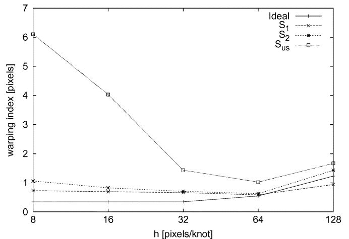
Fig. 6. The dependence of the geometrical error on the knot spacing in space ( h ).
